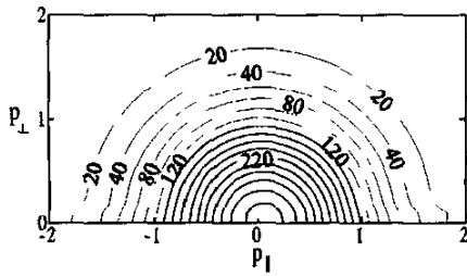
FIG 1 Ion distribution function f_i(x, P_{\perp}, P_{\parallel}) in units of 10^{-2} n_0 / v_i^3 is shown as function of dimensionless perpendicular, P_{\perp} , and parallel, P_{\parallel} , velocities, x = 77.35
