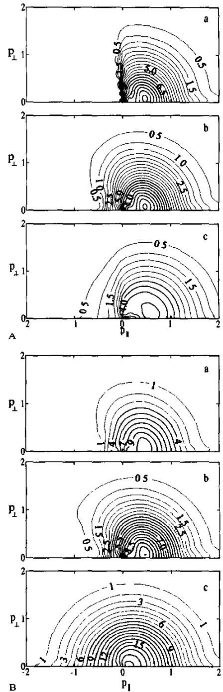
FIG 2 Time evolution of ion distribution function f_i(x, P_{\perp}, P_{\parallel}, t) in units of 10^{-2} n_0 / v_i^3 for two distances from the electrode [(A), x = 0.124 , (B), x = 0.681 ], is shown for times t_i equal to (a) 0.08, (b) 0.23, (c) 0.77, \epsilon = 2.32
