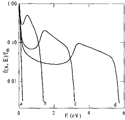
FIG 6 Space- and energy-dependent ion distribution function f_i(x, E) normalized to the maximum f_m . The positions x are equal to (b) 1.1, (c) 0.8, (d) 0.5 for \epsilon = 8 \times 10^{-3} . Maxwellian distribution is shown by curve a
