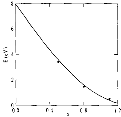
FIG 7 The dependence of ion energy versus distance from the electrode for \epsilon = 8 \times 10^{-3} . Solid line represents free-fall model, while symbols corresponds to the energies of the second peaks of the curves in Fig 6
