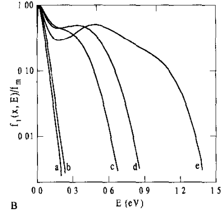
FIG 8 Space- and energy-dependent ion distribution function f_i(x, E) normalized to the maximum f_m for two distances to the electrode [(A), x=0.5 , (B), x=1.1 ], is shown for \epsilon equal to (b) 0.773, (c) 0.024, (d) 0.014, (e) 0.008. Maxwellian source distribution is shown by the curve a
